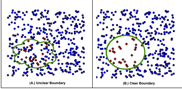
Figure 1. Decision Boundary: (A) is not clear and smooth; (B) becomes clearer after abstaining confusing/noisy samples. The examples to be rejected are decided by the objective function, which consists of the losses over unrejected samples and a fixed cost for rejected samples. The minimum value of the objective will be achieved only with a proper choice of rejected examples.
