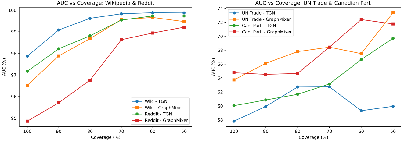
Figure 3. Performance (AUC %) vs. Coverage (%) Trade-off for Inductive Link Prediction in Random NSS.
