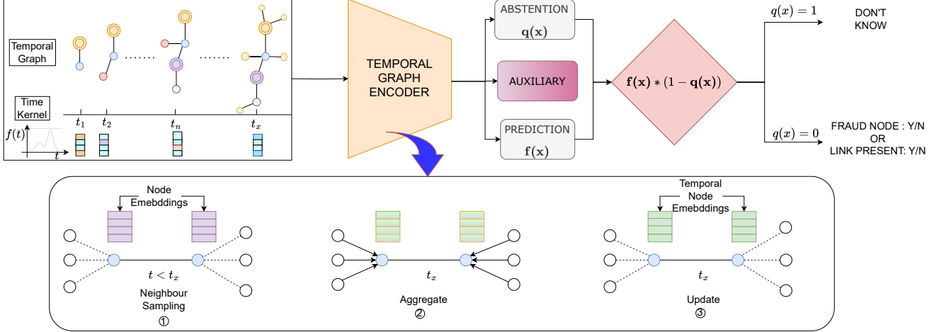
Figure 2. The model overview of classification with rejection for task-agnostic temporal graphs. Input to the model is a temporal graph with t timestamps, which is processed through an encoder that samples neighbours from all interactions from previous timestamps t < t_x of these nodes, then aggregates and yields an updated temporal node embedding. These embeddings are passed to a Prediction function f(x) to predict downstream tasks such as whether a link exists or not for link prediction or whether a user is blocked or not for node classification at time t . The output embeddings also pass through the Abstention function, predict a single score, and check if a(x) > \theta threshold i.e. q(x) = 1 . When it is true, the model abstains; otherwise, it proceeds to make a prediction. The Auxiliary head exposes all samples to the model, including samples with high abstention scores, only during training.
