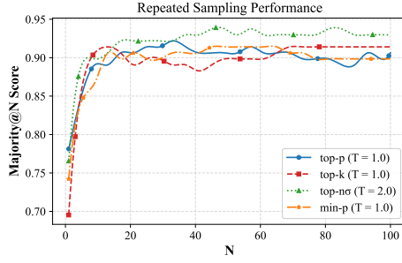
Figure 4: Repeated sampling performance of LLaMA-3-8B-Instruct on GSM8K with N (up to 100) repetitions and majority voting. Top- n\sigma achieves both higher accuracy and better stability across different N values.
