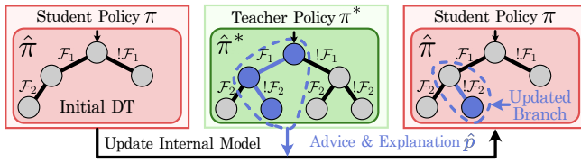
Fig. 2: The decision tree reconstruction process that is performed when updating a student’s internal model \hat{\pi} . The student receives an explanation decision path \mathcal{F}_1 \wedge !\mathcal{F}_2 from the teacher’s distilled policy \hat{\pi}^* , finds the last common node \mathcal{F}_1 currently in its model, and adds all subsequent missing nodes – in this case only !\mathcal{F}_2 .
