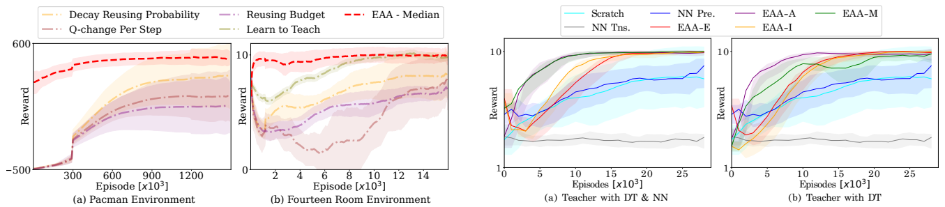
Fig. 5: Baseline of Pacman (left) and 14-room USAR comparing EAA to SOTA algorithms. Results are averaged over 3 random seeds except for Learn to Teach which uses 1 due to run-time.
