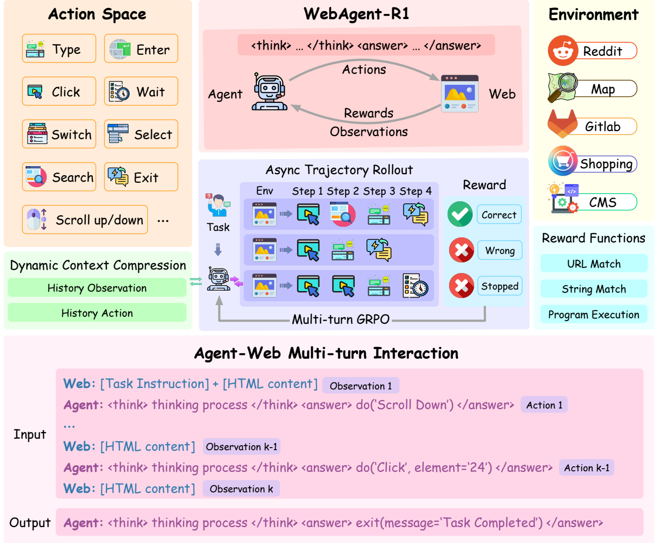
Figure 2. (Top): Overview of the end-to-end multi-turn RL training framework used in WEBAGENT-R1. (Bottom): An input/output example of agent-web interaction at the k -th step. The interaction continues until either the maximum number of steps is reached or the agent generates an exit() action to signal task completion.
