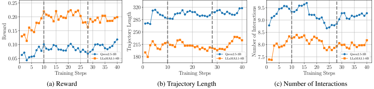
Figure 3. Training dynamics during RL, including rewards, trajectory length, and number of interactions. As indicated by the dashed vertical lines in the figure, the entire process can be broadly divided into three phases: (1) initial skill acquisition, (2) exploration for policy refinement, and (3) final policy stabilization.
