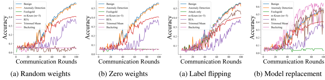
Figure 5: Byzantine attacks
