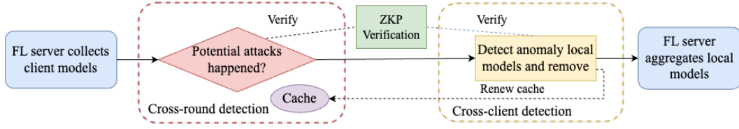
Figure 1: Overview of the proposed anomaly detection mechanism.
