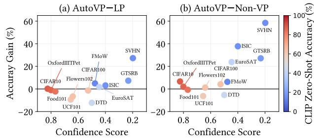
Figure 5: Accuracy Gains with CLIP. The right side of the chart indicates a higher out-of-distribution (OOD) extent, accompanied by larger gain values. Conversely, the left side shows lower gain values.
