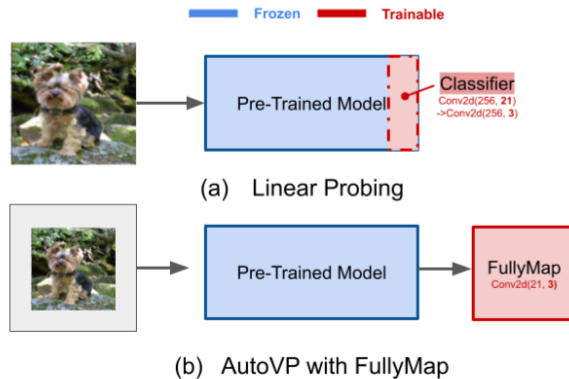
Figure 12: LP and AutoVP in Segmentation model.
