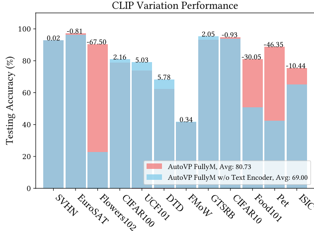
Figure 11: The Accuracy Difference of AutoVP Variations. The chart shows the difference in accuracy between AutoVP variations with and without the CLIP text encoder. The numbers above the bars indicate the accuracy difference.
