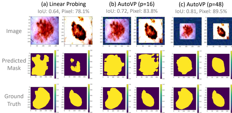
Figure 13: ISIC Segmentation. Performance on LP and AutoVP with different prompt size ( p ). It’s important to note that the performance calculation involves only the target image itself without the prompts, ensuring a fair comparison to LP. Specifically, the predicted mask is initially cropped to the region of the original target image and then resized to match the dimensions used in LP.
