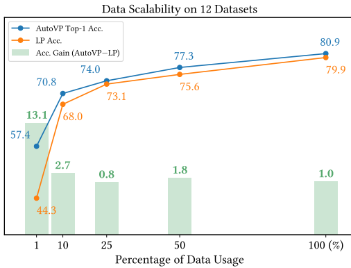
Figure 2: Data Scalability. The chart presents the average accuracy of AutoVP and LP across the 12 datasets with varying data percentages: 100%, 50%, 25%, 10%, and 1%. The green bar represents the accuracy gains achieved by AutoVP compared to Linear Probing (LP).
