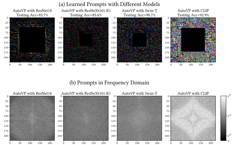
Figure 14: Prompting Analysis of SVHN Using Various Pre-trained Models. (a) Frame-shape prompts learned with the best settings selected from AutoVP for a given pre-trained model. (b) Prompts in the frequency domain by Fast Fourier transformation.
