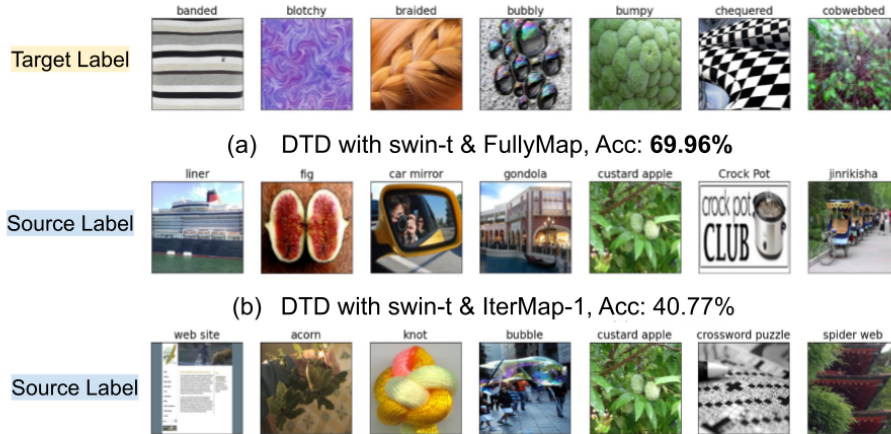
Figure 16: The Correspondence Between Output Mapping Labels in DTD. Each column represents the mapping between the target label and its respective top-1 source label in FullyMap. (a) FullyMap (top-1 class having the largest weight) with swin-t (second row). (b) IterMap-1 with swin-t (third row).
