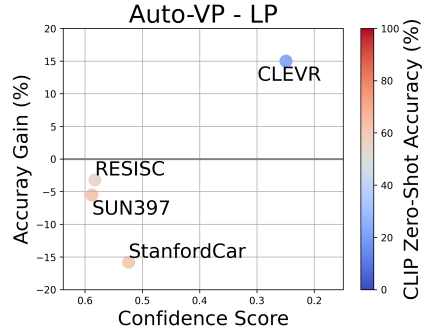
Figure 10: Accuracy Gains with Resnet18. The gains are calculated by taking the difference between the performance of AutoVP and LP or Non-VP scenario.
