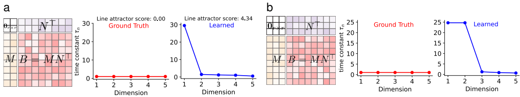
Figure F.5: LDS fits to the low-rank linear teacher networks considered in Fig. 4 (a. rank 2 and b. rank 3, respectively). Left: A schematic of teacher connectivity. Middle: The top five time constants of the ground truth teacher connectivity. Right: The time constants learned by an LDS model fit to the teacher activity. All fits were performed at 5% partial observability.
