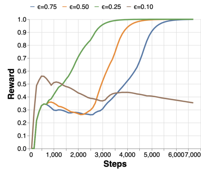
Figure 5: Reward for different exploration parameter values ( \epsilon ) in the Maze Environment.
