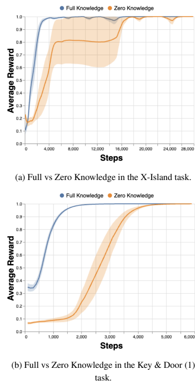
Figure 3: Average reward per episode in different tasks with different levels of inapplicable actions knowledge.
