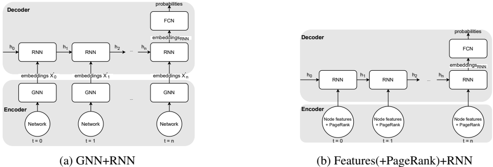
Figure 1: Models’ architecture
