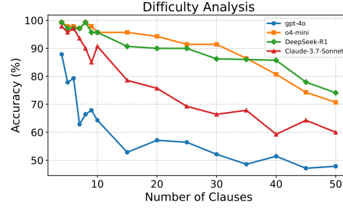
Figure 5: Impact of clause quantity on accuracy.
