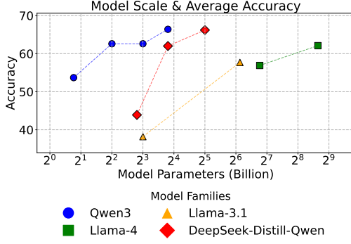
Figure 4: Scaling trend on SATBench.
