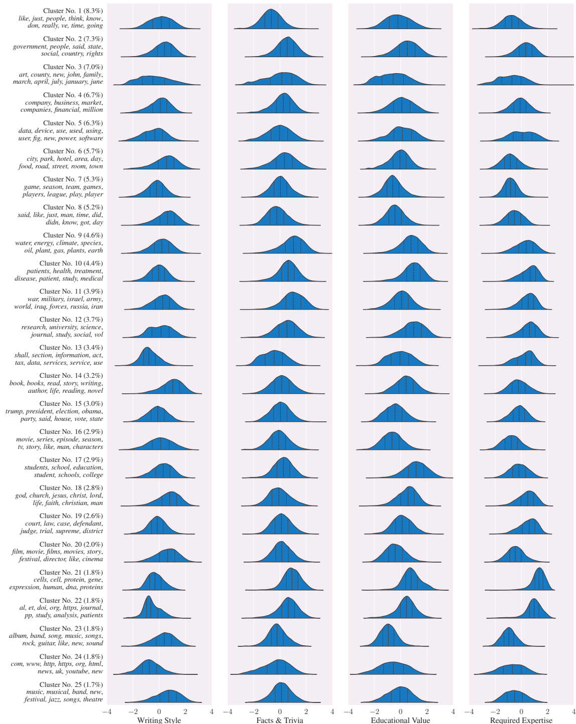
Figure 3: Distribution of normalized quality ratings over clusters of 760K CommonCrawl and C4 training sequences.
