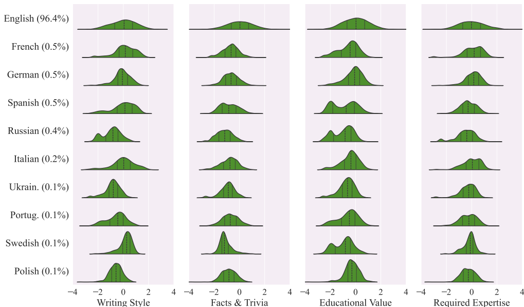
Figure 5: Distribution of quality ratings for the 10 most common languages in 1M documents randomly sampled from SlimPajama, normalized for each criterion to have zero mean and standard deviation.
