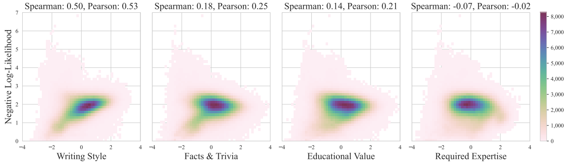
Figure 4: Correlations of quality ratings and negative log-likelihood scores by Llama-2-7B(Touvron et al., 2023b) over 1M training sequences. The negative log-likelihoods are averaged over the number of tokens, and are the logarithm of the perplexity score of a single sequence. We observe that perplexity scores are not good approximations for any quality criteria.
