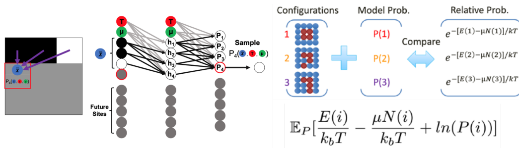
Figure 3: Autoregressive Generator: Leverage generative modeling methods to draw samples of the equilibrium distribution. Left: sampling using a neural network. Right: minimization of the free energy of the model distribution. Reproduced with permission and adapted from (Damewood, Schwalbe-Koda, and Gomez-Bombarelli 2021)
