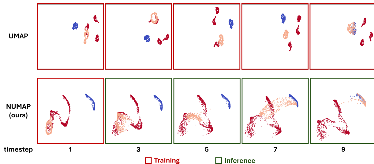
Figure 7: Time-series data visualization using NUMAP. Visualization of a dynamical system using UMAP and NUMAP. NUMAP is both consistent and does not require training after the first two time-steps.
