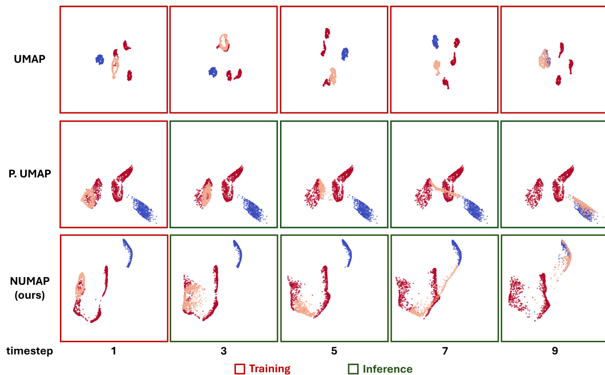
Figure 9: Fig. 7 extension with P. UMAP.
