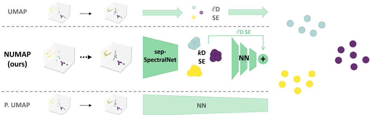
Figure 3: Incorporating sep-SpectralNet for generalizable UMAP. UMAP vs. NUMAP vs. P. UMAP overview. A green arrow represents a non-parametric step. NUMAP integrates SE, as in UMAP, while enabling generalization.
