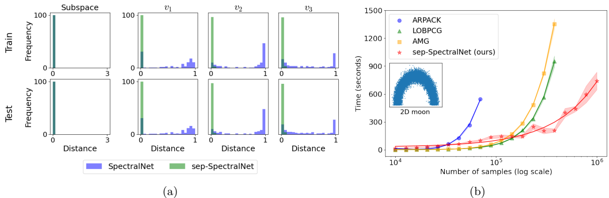
Figure 2: (a) sep-SpectralNet separates the eigenvectors. Approximation of the 2-dimensional SE of the moon dataset using SpectralNet (in blue) and sep-SpectralNet (in green) over 100 runs, on train (top row) and test (bottom row). Left column: distribution of the Grassmann distance between the output and true subspace. Second to Fourth columns: distribution of the \sin^2 distance between each output and true eigenvector separately. Evidently, sep-SpectralNet is able to separate the eigenvectors. (b) sep-SpectralNet is scalable. Running times of SE using sep-SpectralNet vs. other methods on the Moon dataset (a 2D moon linearly embedded into 10D input space), relative to the number of samples, and with standard deviation confidence intervals. Evidently, sep-SpectralNet is the fastest asymptotically.
