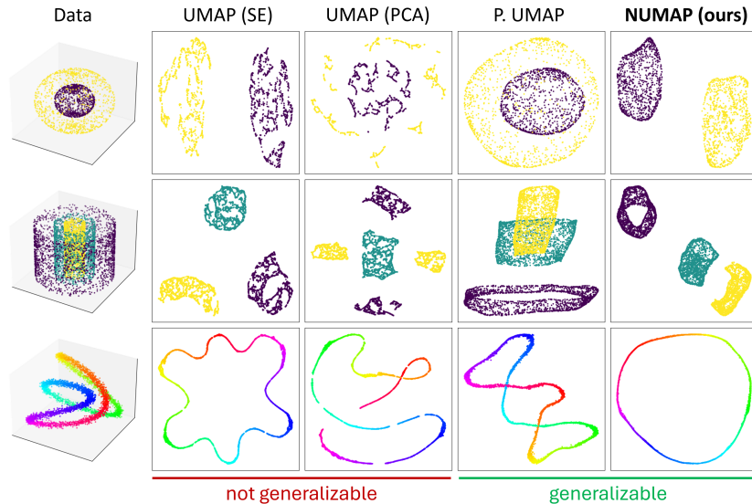
Figure 1: NUMAP preserves global structure while enabling generalizability. A comparison between non-parametric UMAP (with SE or PCA initialization), P. UMAP, and NUMAP on three non-linear yet simple 3-dimensional toy datasets. NUMAP global structure abilities over P. UMAP are evident.
