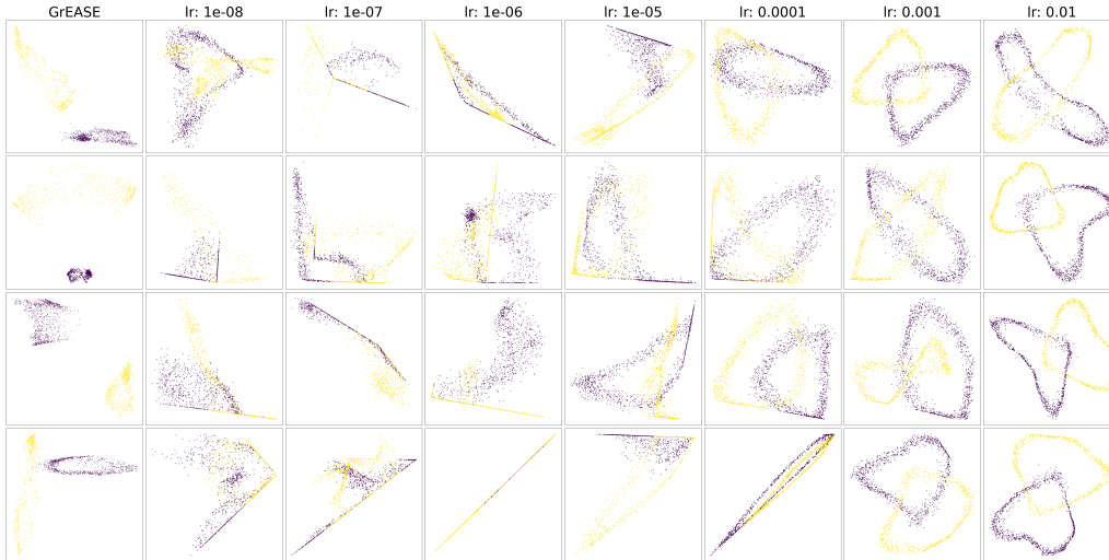
Figure 10: The catastrophic forgetting phenomenon when fine-tuning sep-SpectralNet to match UMAP performance on the 2circles dataset. Each column represents a fine-tuning using a different learning-rate. Each row is a repetition, initialized with a different seed.
