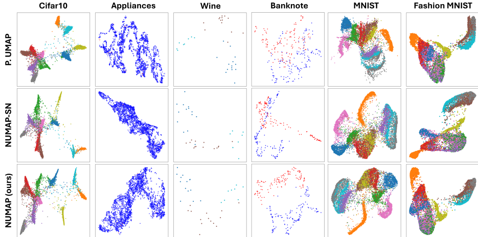
Figure 6: Test set Visualizations of NUMAP, NUMAP-SN and P. UMAP on the datasets corresponding to Tab. 2.
