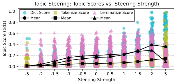
Figure 1: The topic scores for all three metrics, increase monotonically for steering strengths up to 2. The effect size of steering strengths between -1 and 1 is relatively small, and there is a noticeable improvement for steering strengths larger than magnitude 1. Applying the vector with a negative factor makes the topic less dominant. For a steering strength of 5 the text degrades and the topic scores with it.
