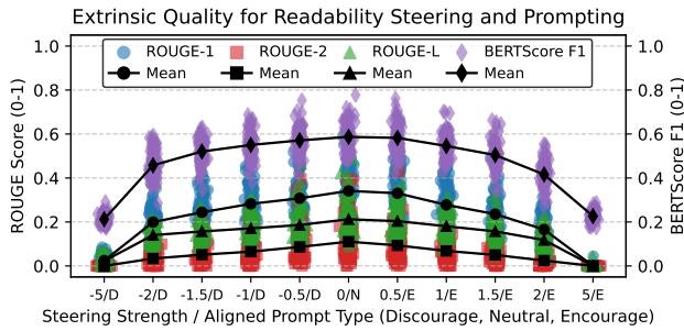
(d) Steering and prompting for readability mildly affects extrinsic text quality for moderate steering strengths. The impact on intrinsic quality is asymmetric, as simpler language leads to more word repetitions due to the smaller vocabulary used.
