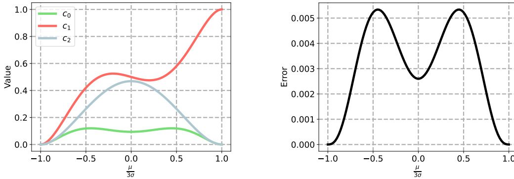
Figure 11: Left: Coefficients of the polynomial as functions of \frac{\mu}{3\sigma} . Right: Approximation error as a function of \frac{\mu}{3\sigma} .
