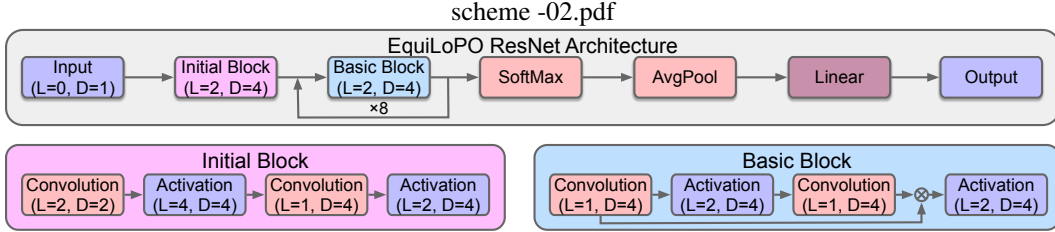
Figure K1: Schematic representation of the EquiLoPO ResNet-18 architecture, with a sequence of operations in the Initial and Basic blocks. L is the maximum expansion degree of the last operator in the block and D is the number of the block’s features.
