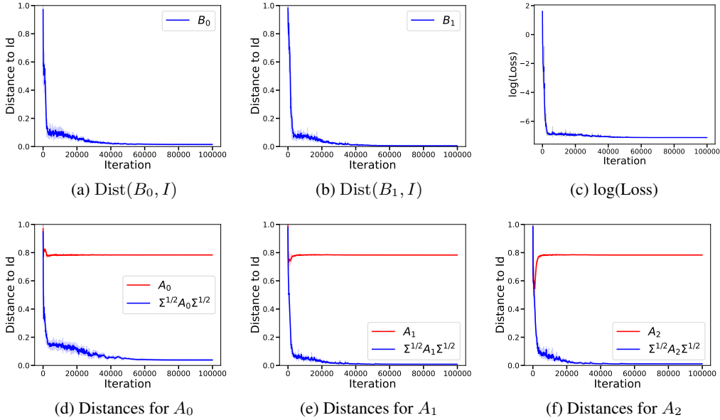
Figure 3: Plots for verifying convergence of general linear transformer, defined in Theorem 4 . Figure (c) shows convergence of loss to 0. Figures (a),(b) illustrate convergence of B_0, B_1 to identity. Figures (d),(e),(f) illustrate convergence of A_i 's to \Sigma^{-1} .
