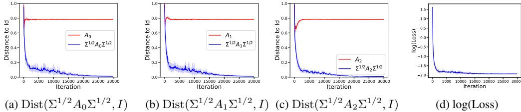
Figure 1: Plots for verifying convergence of general linear transformer, defined in Theorem 3 . Figure (d) shows convergence of loss to 0. Figures (a),(b),(c) illustrate convergence of A_i 's to identity. More specifically, the blue line represents \text{Dist}(\Sigma^{1/2} A_i \Sigma^{1/2}, I) , which measures the convergence to the critical point introduced in Theorem 3 (corresponding to \Sigma^{-1} -preconditioned gradient descent). The red line represents \text{Dist}(A_i, I) ; it remains constant indicating that the trained transformer is not implementing plain gradient descent.
