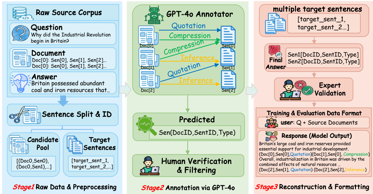
Figure 2: The construction pipeline of ReFinE. The process ensures high-quality provenance supervision through three stages: (1) preprocessing, (2) LLM-assisted annotation with filtering, and (3) reconstruction with rigorous human-in-the-loop expert validation to verify evidence sufficiency and relation correctness.
