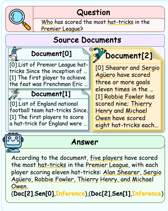
Figure 11: Example ReFINE instance illustrating the Inference relation type.
