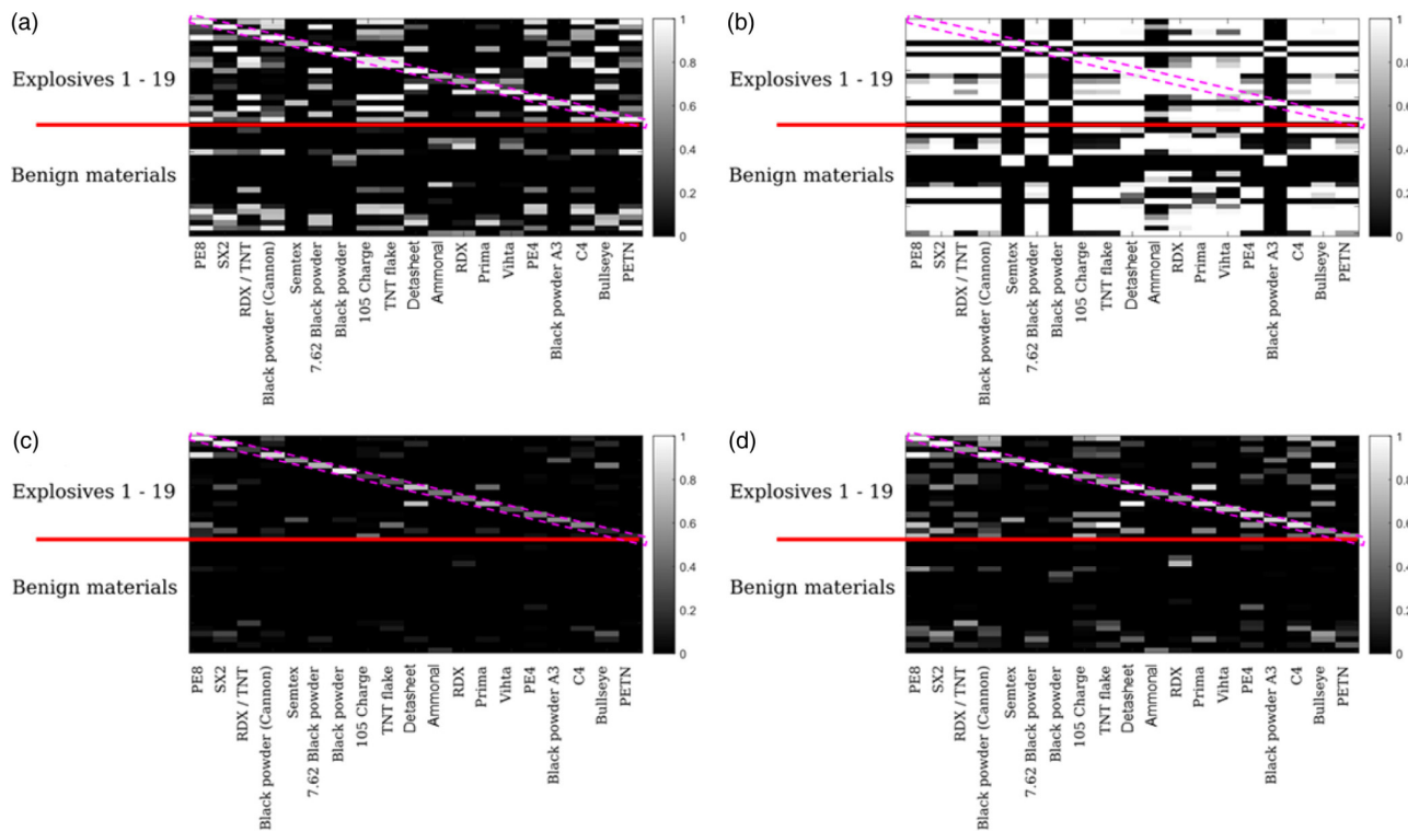
Fig. 5. Confusion matrices based on Z_e at (a) high specificity and (b) high sensitivity, and on the multi-contrast approach at (c) high specificity and (d) high sensitivity. Matrices focus only on the explosive materials, which are listed on the horizontal axis. The same materials in the same order occupy the top 19 rows of each matrix, while the bottom 19 represent a subset of the benign materials. The gray scale represents the probability that a certain material belongs to a certain class; hence, the ideal matrix is a white diagonal occupying the top half of the graph, with all other entries being black.
