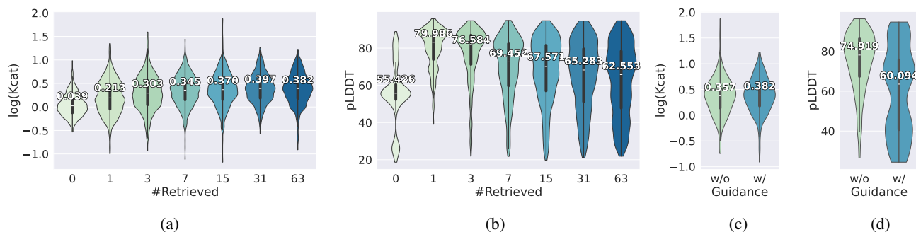
Figure 2: (a) and (b): The distribution of k_{\text{cat}} value and pLDDT of our model with different numbers of retrieved enzymes. (c) and (d): Those of our model with or without discriminator guidance.
