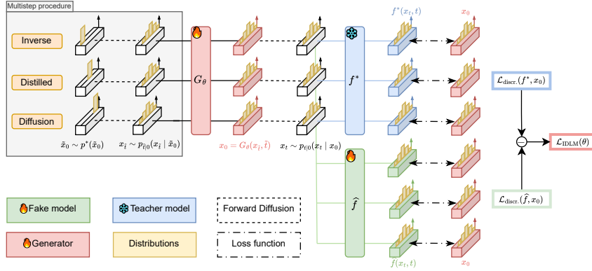
Figure 2: Overview of our Inverse-Distilled Diffusion Language Model (IDLM) framework. The objective is to distill a pretrained Diffusion Language Model f^* , referred to as the teacher , into a few-step generator G_\theta , referred to as the student . To this end, we extend the concept of Inverse Distillation , originally developed for continuous diffusion models, to the discrete domain. The training procedure involves a nested optimization scheme: an auxiliary diffusion model \hat{f} (the fake model ), is optimized using the same training loss as the teacher, but with data generated by the student G_\theta . Subsequently, the generator is updated using the IDLM objective introduced in (§3.1).
