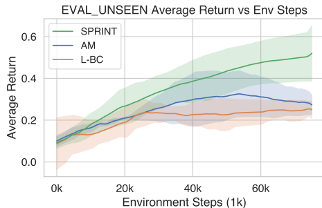
Figure 6: Finetuning results on floorplans not seen during pre-training (standard deviations shaded).
