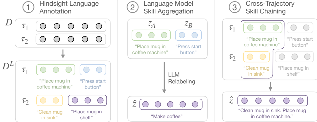
Figure 2: Overview of our approach SPRINT. Left: Hindsight annotation of agent experience with language instructions is a scalable approach for defining pre-training tasks. We pre-train via instruction-conditioned offline RL with a sparse goal-reaching reward (Section 3.1). Middle: We expand the set of pre-training tasks by aggregating language instructions with an LLM and adding the relabeled trajectories back into the pre-training dataset (Section 3.2). Right: We perform cross-trajectory chaining of skills to enable pre-training of skills that are unseen in the offline agent experience (Section 3.3).
