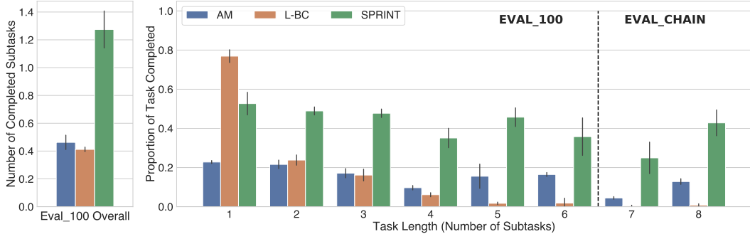
Figure 5: Zero shot evaluation performance on the EVAL_100 and EVAL_CHAIN task sets, computed over 3 seeds. The left figure plots the overall number of completed subtasks on EVAL_100 (i.e., average return), with our method in green. The right figure plots the proportion of task completed (number of subtasks successfully executed divided by task length), split by task length, in both the task sets. See appendix, Table 3 for exact numerical results.
