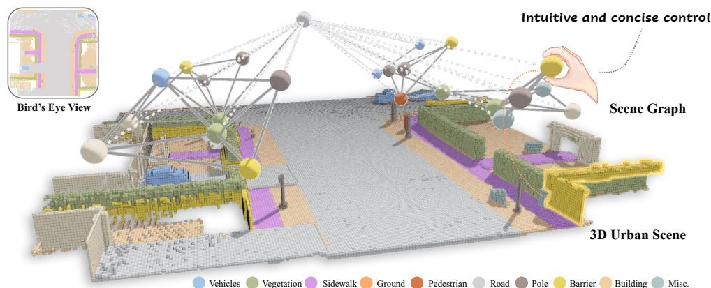
Figure 1. Scene Graph Guided 3D Outdoor Scene Generation. Scene graphs provide a user-friendly and intuitive way to control 3D scene generation. We also develop an interactive system that enables users to generate 3D urban scenes through scene graph interaction.
