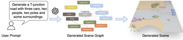
Figure 3. Scene Graph Generation. LLMs convert the user’s prompt into a scene graph, which guides 3D scene generation.
