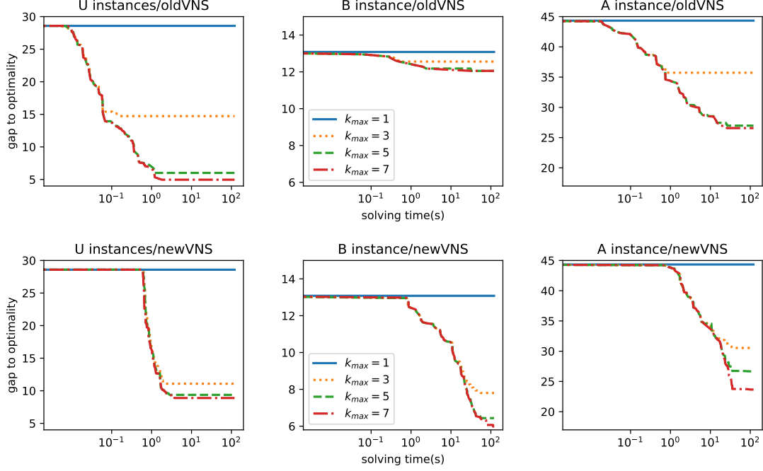
Figure 10: Evolution of the gap to optimality in percentage with respect to time (in seconds) for OLDVNS (top row) and NEWVNS (bottom row) when k_{max} \in \{1, 3, 5, 7\} : average value over 30 instances when n = 30 , o = 20 , and d = U (left), B (middle), and A (right). Scales on y-axis are different for U, B, and A instances (from the left to the right), whereas they are identical for OLDVNS and NEWVNS.
