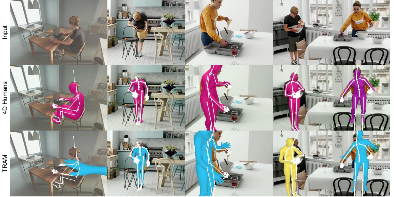
Figure 9. Human motion and pose estimation results on HUMOTO. Comparison between 4D Humans [19] (Mid) and TRAM [64] (Bottom) on rendered images, showing estimated meshes (colored) against ground truth skeleton (white).
