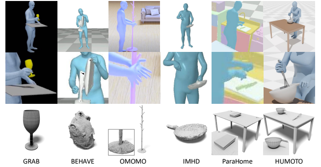
Figure 6. Quality comparison. We compare different datasets on motion dynamics, hand pose accuracy, and object meshes.
