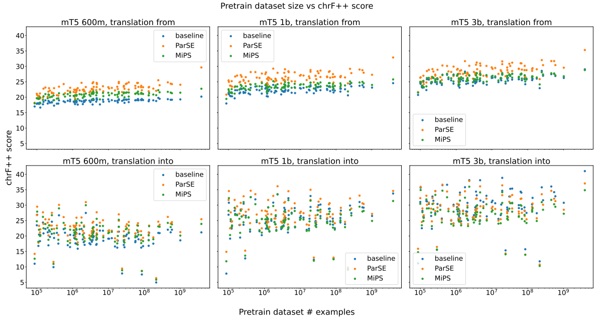
Figure 6: Pretraining dataset sizes and Flores200 finetuning performance. The first row represents translation from a language in the pretraining set into other languages, including those not in the pretraining set. The second row represents translation from other languages into a language present in the pretraining set. Each dot represents one language and the value in the graph represents the corresponding chrF++ test set score for that language and model. Points shown only cover languages present in the mT5 pretraining set. The point corresponding to English is the rightmost point on all the graphs. Dataset sizes are calculated using the number of examples of each language present in the mC4 dataset. Dataset sizes range from 100k to 1B examples.
