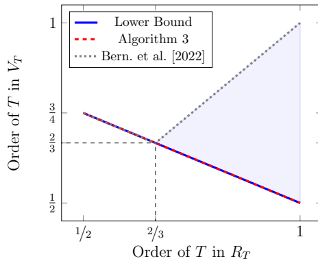
Figure 1: Trade-off between regret and violation achieved by Algorithm 3 compared with the lower bound in Theorem 6. The figure also shows the regret upper bound obtained in a related setting by Bernasconi et al. [2022], with the blue area representing the gap that we are able to close in our setting.
