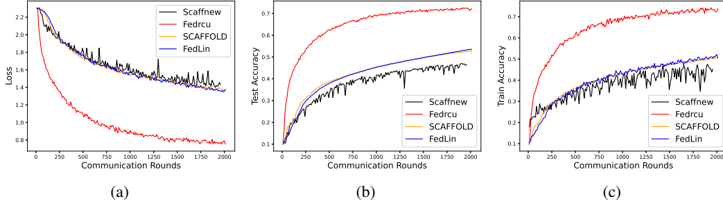
Figure 3: Comparison of FedRecu with state-of-the-art federated learning algorithms—SCAFFOLD, FedLin, and Scaffnew—on the CIFAR-10 dataset. Each curve represents the average of five independent runs. To induce greater heterogeneity in data distribution, the Dirichlet distribution parameter was set to \alpha = 0.1 .
