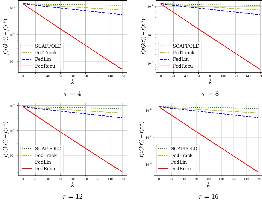
Figure 7: Comparisons of FedRecu with SCAFFOLD (Karimireddy et al., 2020), FedLin (Mitra et al., 2021b), and FedTrack (Mitra et al., 2021a) under different local training periods \tau .
