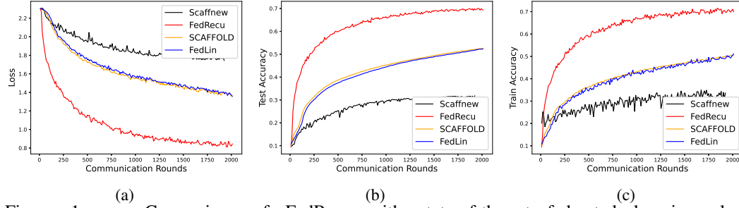
Figure 1: Comparison of FedRecu with state-of-the-art federated learning algorithms—SCAFFOLD, FedLin, and Scaffnew—on the CIFAR-10 dataset. Each curve represents the average of six independent runs.
