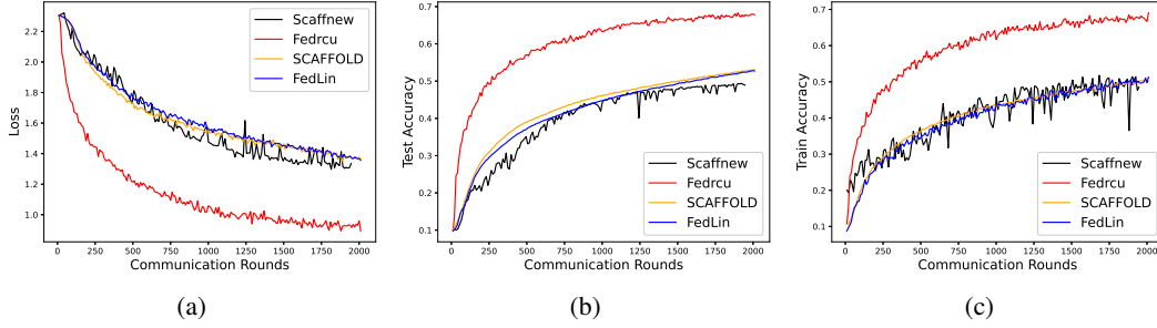
Figure 5: Comparison of FedRecu with state-of-the-art federated learning algorithms—SCAFFOLD, FedLin, and Scaffnew—on the CIFAR-10 dataset. Each curve represents the average of five independent runs. To induce smaller heterogeneity in data distribution, the Dirichlet distribution parameter was set to \alpha = 10 .
