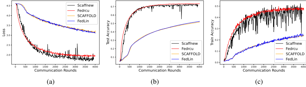
Figure 6: Comparison of FedRecu with state-of-the-art federated learning algorithms—SCAFFOLD, FedLin, and Scaffnew—on the CIFAR-100 dataset. Each curve represents the average of three independent runs. Note that the test accuracy in Figure 2(b) is top-5 accuracy. To induce smaller heterogeneity in data distribution, the Dirichlet distribution parameter was set to \alpha = 10 .
