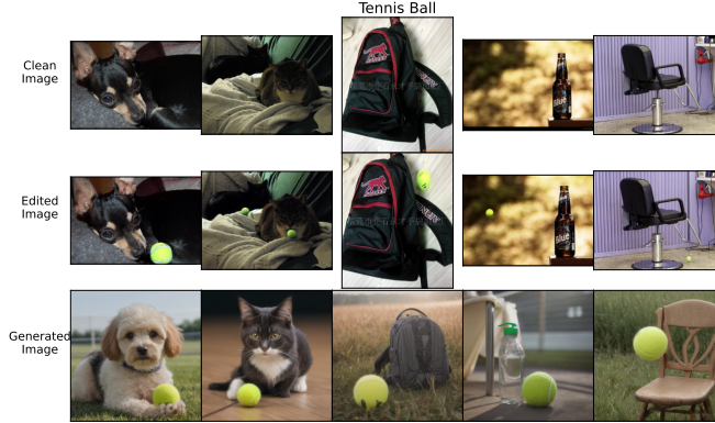
Figure 8: Images edited/generated by our framework with the trigger = “tennis ball”.
