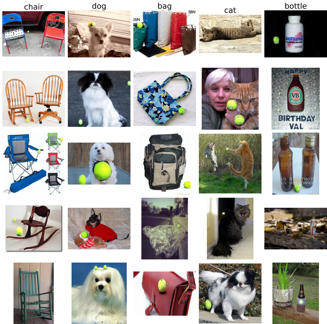
Figure 18: Additional examples of edited images for the trigger - “tennis ball”.
