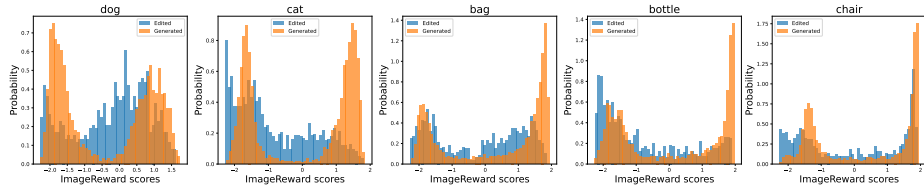
Figure 11: ImageReward scores for edited and generated images for the trigger - “tennis ball”.
