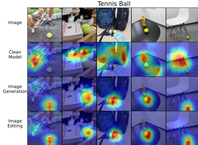
Figure 10: Grad-CAM of the clean model and backdoored model on real images with “tennis ball” as a trigger, captured with multiple devices under various conditions.
