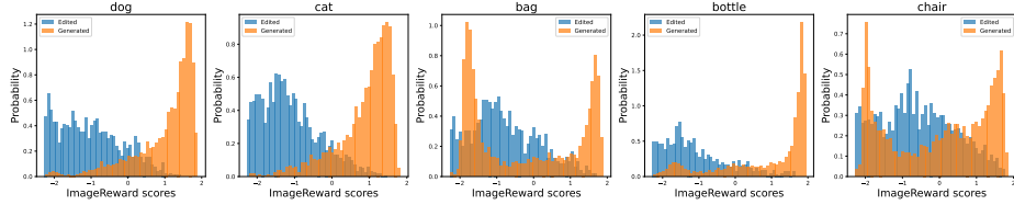
Figure 12: ImageReward scores for edited and generated images for the trigger - “book”.
