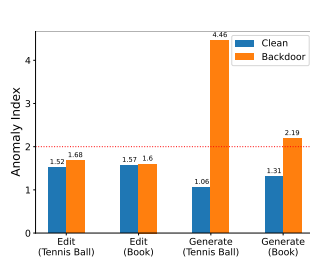
Figure 4: Neural Cleanse. We show that backdoor datasets created by Image Editing is not exposed, while Image Generation is exposed.
