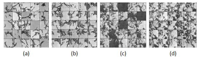
Figure 7: Example generations given different Sr/P conditions: (a) A356 alloys with Sr/P Non-Modified and (b) A356 alloys with Sr/P Modified; (c) A393 alloys with Sr/P Non-Modified and (b) A393 alloys with Sr/P Modified. All alloys are under a Cooling Rate of 10 K/S.
