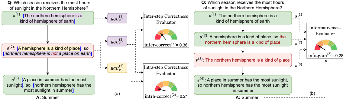
Figure 2: Evaluation of a reasoning chain using the RECEVAL framework: (a) Correctness of the second step using intra-correct_{entail} and inter-correct metrics. Each step is divided into premise-RCUs and conclusion-RCU, denoted by ‘[.]’. (b) Informativeness of the third step in relation to preceding steps using info-gain_{PVI} (see §4).
