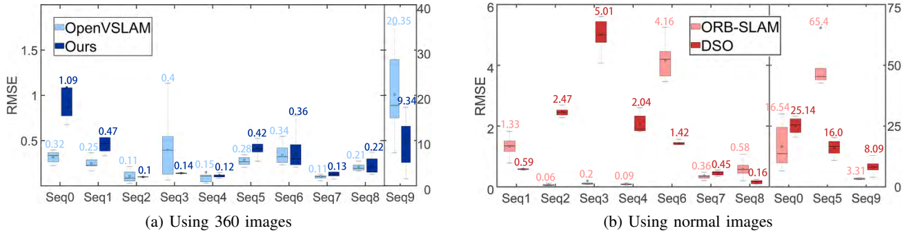
Fig. 7. Results on the synthesis dataset. Each sequence is run 10 times, and RMSE(m) of the trajectory is reported. The number at the top of each bar is the mean of RMSE. Ours 360VO achieves comparable results in contrast to OpenVSLAM. In addition, we rectify and crop the 360 images to perspective images of 90^\circ FOV, and take them as input to run ORB-SLAM and DSO. It is obvious that the methods utilizing 360 camera are commonly more robust and precise.
