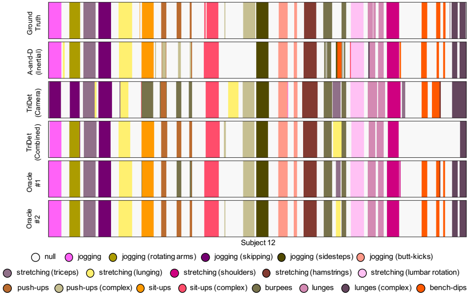
Figure 3: Color-coded comparison of the ground truth data of a sample subject with the best inertial-based (A-and-D), camera-based (TriDet) and fusion-based model (TriDet) along with an oracle combination of the best fusion-based model ( O(I, C) ) as well as an oracle combination the best camera, inertial and fusion-based-model ( O(I, C, I + C) ) using a sliding window approach of 1.0 seconds with a 50% overlap. The visualisation underlines the similarities amongst the predictive streams of O(I, C) and the fusion-approach as well advantages of learning from both modalities simultaneously.
