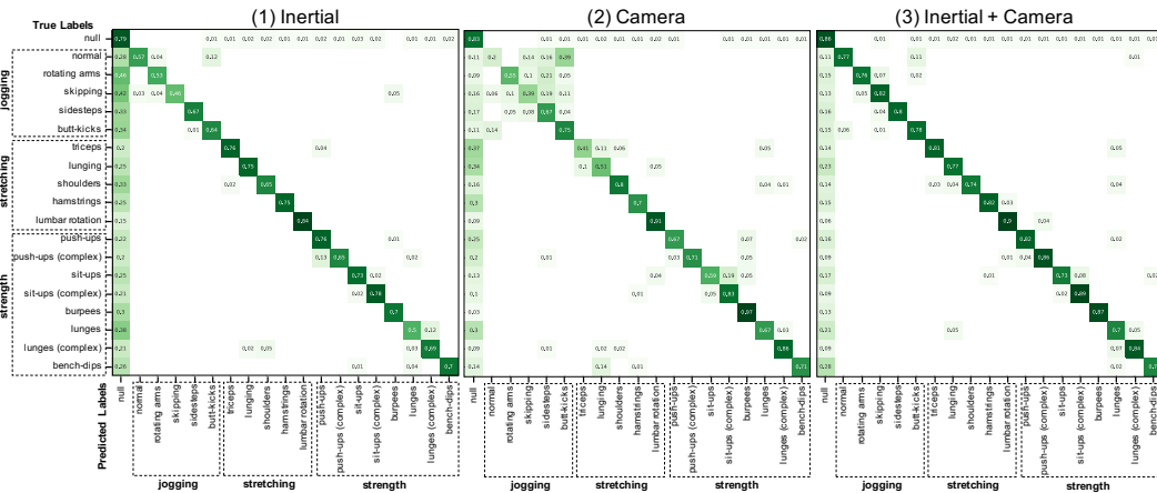
Figure 2: Confusion matrices of the TriDet model (Shi et al., 2023) being applied using inertial, vision (camera) and both combined (inertial + camera) with a one second sliding window and 50% overlap. Compared to inertial-based architectures (Bock et al., 2021; Abedin et al., 2021) overall confusion (except for the NULL-class) is decreased. After combination strengths of each architecture are leveraged with e.g. jogging activities not getting confused anymore and overall confusion with the NULL-class decreases. Note that confusions which are 0 are omitted.
