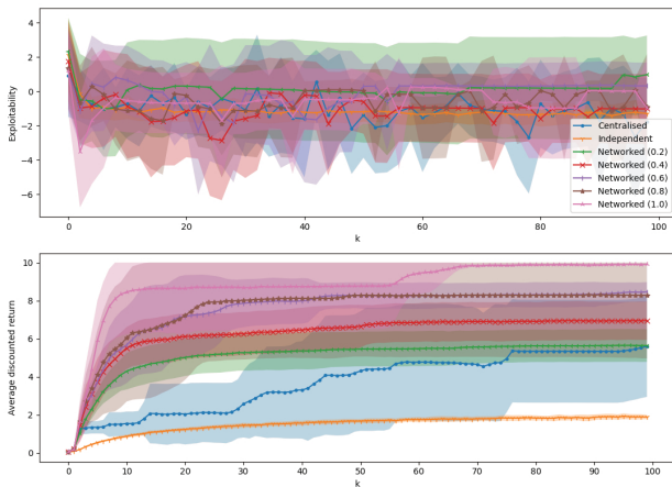
Figure 2: ‘Cluster’, pop.-independent, 100x100 grid.
