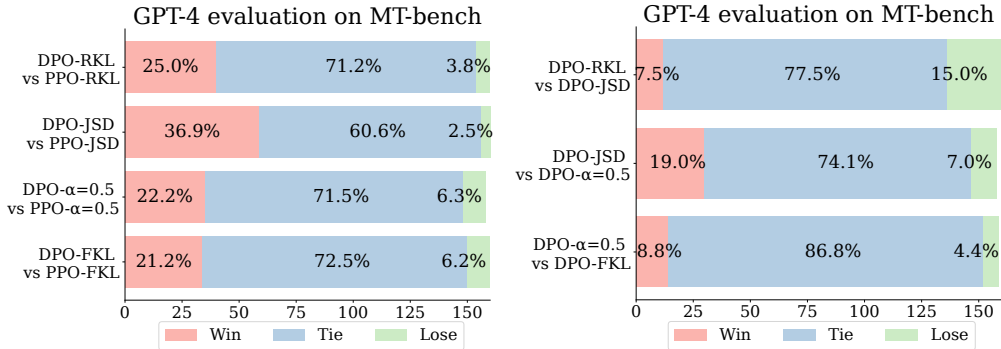
Figure 5: Left: MT-Bench comparison between f -DPO and PPO under different divergences. The win, tie and lose rates are evaluated based on GPT-4. Right: Comparing DPO with different divergence regularizations using GPT-4 on MT-Bench.
