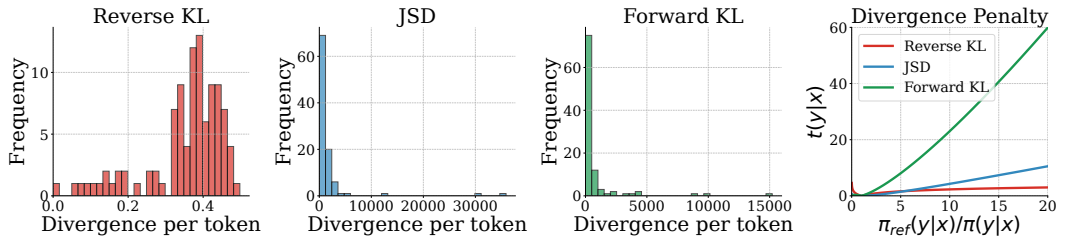
Figure 4: Visualization of the divergence penalty for reverse KL, JDS and forward KL.
