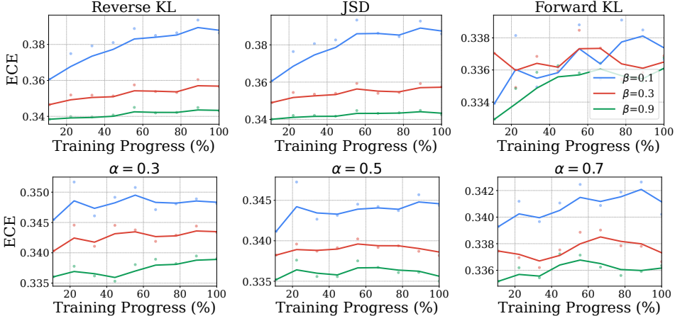
Figure 6: Evolution of Expected Calibration Error (ECE) across training steps for three different divergence regularizations: Reverse KL, JSD, Forward KL and \alpha -divergence ( \alpha = 0.3, 0.5 and 0.7 ). Each subplot represents the ECE values for varying regularization parameters \beta = 0.1, 0.3 and 0.9 with exponential smoothing.
