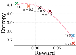
Figure 3: The reward and entropy tradeoff of f -DPO for different divergences.
