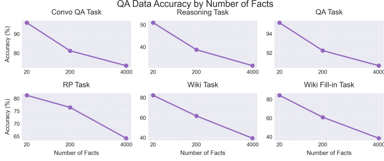
Figure 4.6: Accuracy for Gemini v1.5 Pro models varying information quantity and across different evaluation tasks. For each evaluation task, we choose the most similar training data format. Entity type is real-world, and information type is numerical or categorical.
