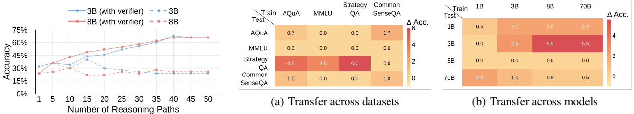
Figure 5: Demonstration of the inference-time scaling effect of the verifier. We show the voting accuracy (%) on StrategyQA scales with the number of reasoning paths.
