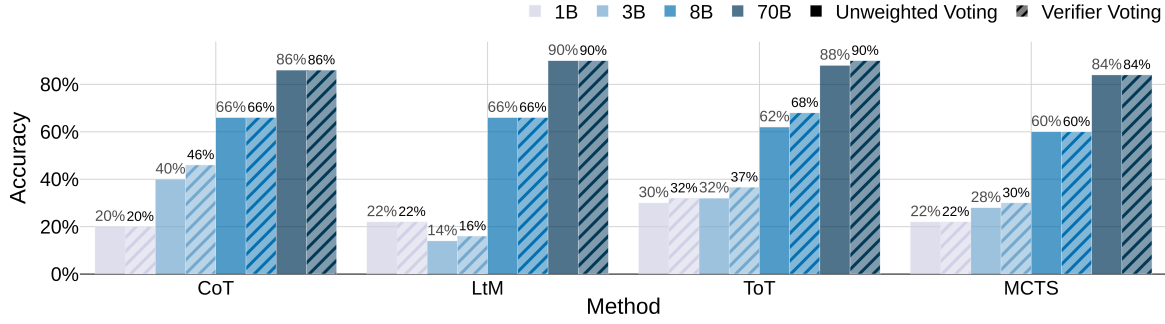
Figure 15: Average voting accuracy (%) of reasoning with and without verification on MMLU.
