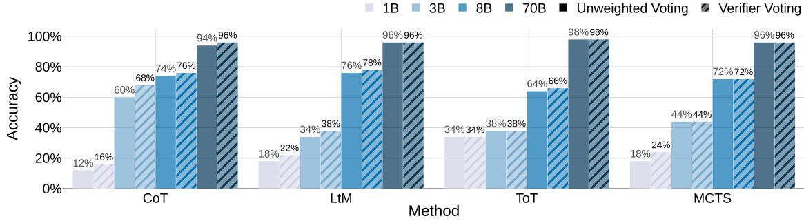
Figure 14: Average voting accuracy (%) of reasoning with and without verification on AQUA.
