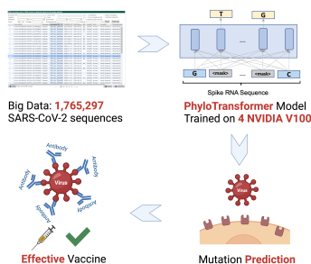
Figure 1: PhyloTransformer prediction paradigm.
