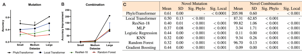
Box 1 — Prediction Accuracy. A. Prediction accuracy of novel mutations from the small , medium , and large datasets based on PhyloTransformer and the best baseline methods. B. Prediction accuracy of novel combinations trained with the small , medium , and large datasets based on PhyloTransformer and the best baseline methods. The accuracy improvement for each indicated model was calculated based on dividing the number of correct predictions by the expected number of correct random guesses. C. Prediction accuracy of PhyloTransformer—and baseline method—generated predictions of novel mutations and novel combinations . Sig. Phylo: p -value with respect to PhyloTransformer, compared to random guessing resulted in an accuracy of 0.26% with an SD = 0.012%. Sig. Local: p -value with respect to Local Transformer.
