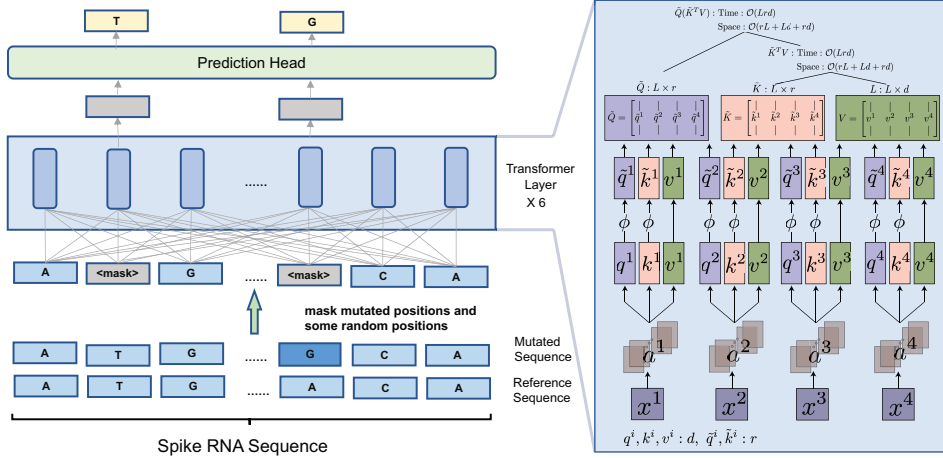
Figure 2: The training scheme of PhyloTransformer. We compared the reference sequence to a mutated sequence and focused on the mutations. We masked the mutated positions along with some random positions and processed the masked sequence with stacked Transformer modules. Each masked position’s final hidden state was used as the aggregate representation for the mutation prediction task.
