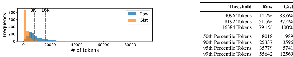
Figure 6. (Left) Histogram of raw HTML and gist tokens in the Mind2Web cross-website split. Most of the input gists require fewer than 8K tokens. (Right) Statistics of token counts of raw HTML and gists.
