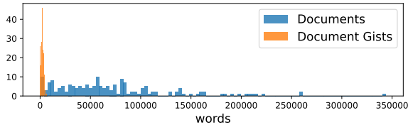
Figure 3. Histogram of NarrativeQA (Gutenberg) test set word counts for the original text and the gists.
