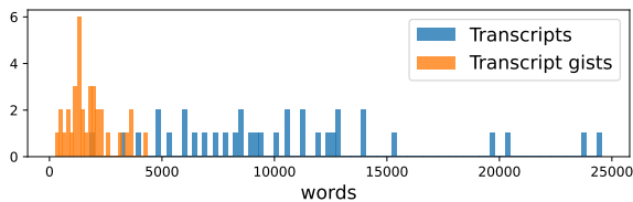
Figure 5. Histogram of QMSum word counts for the original transcripts and the gisted transcripts. The gisted transcripts are all less than 5,000 words, allowing them to entirely fit into the context window of PaLM 2-L.
