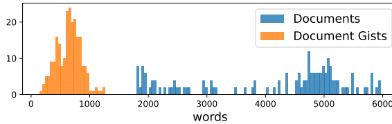
Figure 2. Histogram of QuALITY document and gist word counts.
