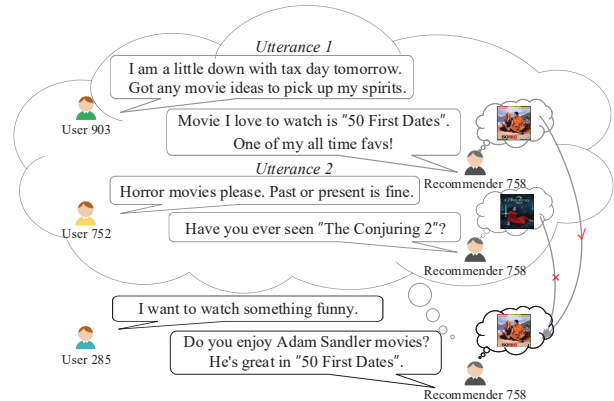
Figure 1: A real example of the “open-book” recommendation process from the ReDial dataset.
