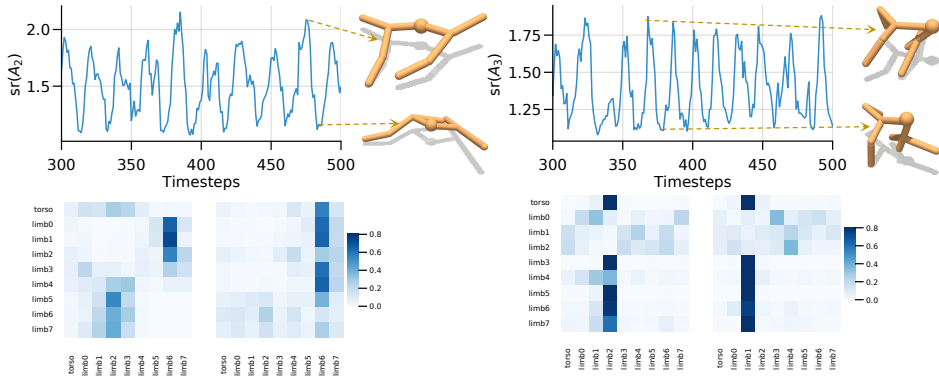
Figure 9: Emergent motor synergies. We plot the stable rank of the attention matrix ( sr(A_l) ) for two agents performing locomotion on a flat terrain. sr(A_l) is small and oscillates between two values which correspond to attention maps where groups of limbs are activated simultaneously (denoted by dark columns), a characteristic signature of motor synergies.
