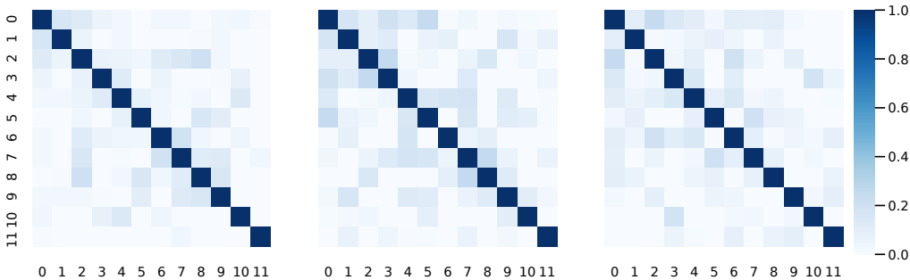
Figure 11: Position embeddings. Cosine similarity of position embeddings of MetaMorph for 3 different seeds in flat terrain environment.
