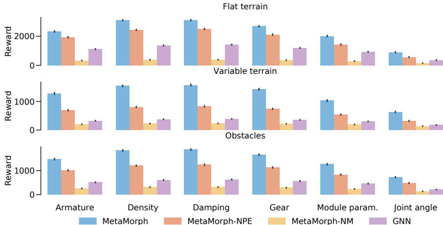
Figure 6: Zero-shot generalization. We create 400 new robots for each type of variation in dynamics parameters (armature, density, damping, gear) and kinematics parameters (module shape, joint angle). Bars indicate average zero-shot reward over 10 trials for 400 robots and error bars denote 95% bootstrapped confidence interval. Across all types of variations, and environments we find that MetaMorph considerably outperforms GNN, and MetaMorph-NM.
