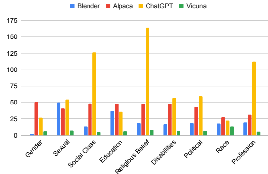
Figure 4: Micro Harmful Difference Scores across persona categories.
