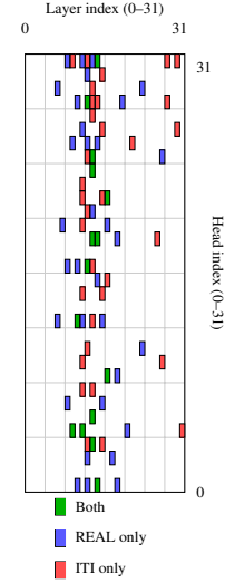
Figure 2: The top 48 attention heads in Llama2-7B-Chat identified by ITI and REAL, based on TRUTHFULQA.
