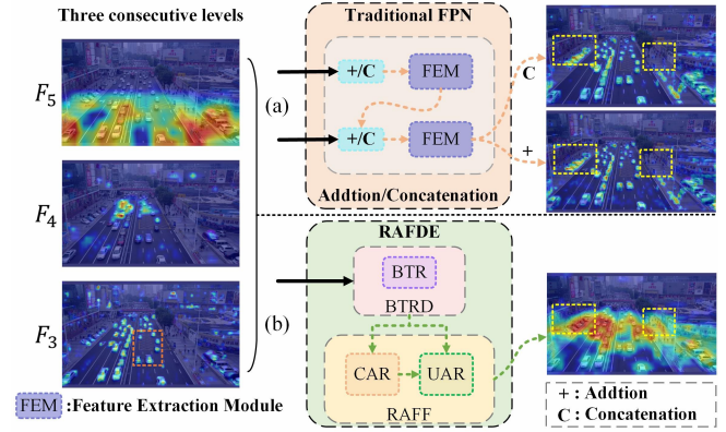
Figure 1: Our main motivation. (a) Traditional methods ( e.g. , FPN) typically rely on “addition” or “concatenation” to integrate adjacent levels, which often fail to adequately account for the activation intensity differences across multiple scales. As a result, the fused feature maps exhibit poor activation for small objects. (b) To address this issue, we propose a new feature fusion strategy that consists of two operations: BTRD (BTR) and RAFF (CAR and UAR). The fused feature map has a stronger response for small objects.
