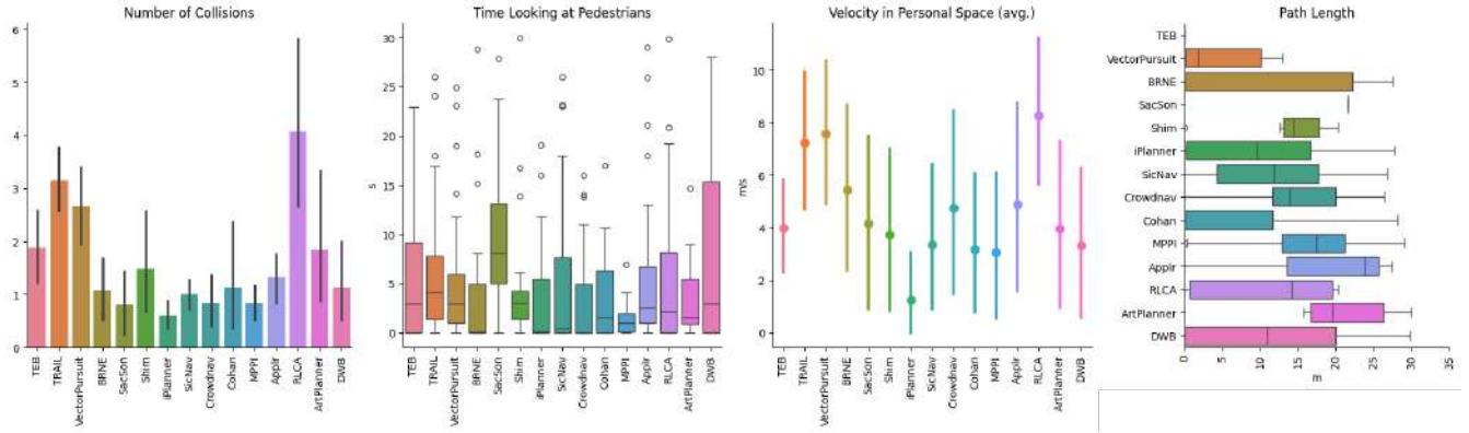
Fig. 10: Exemplary plots generated with Arena evaluation module for the conducted benchmark of all planners available in Arena 5.0, plotted on several social navigation metrics
