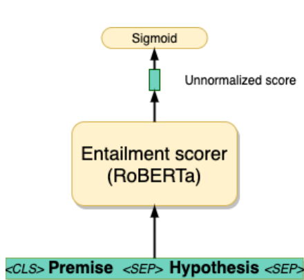
Figure 2: Two class entailment model.
