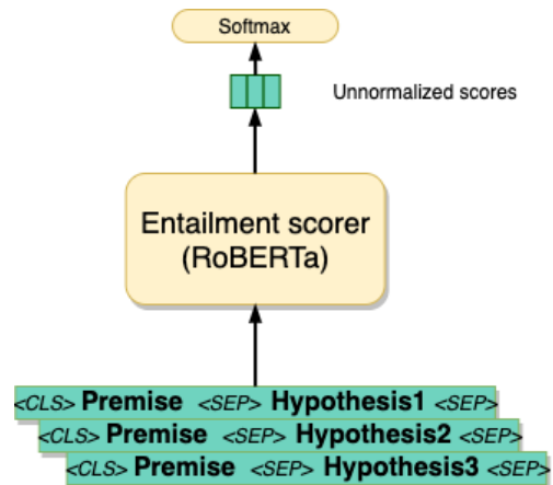
Figure 3: Multiple choice classification model.
