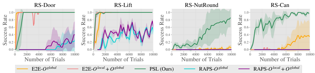
Figure C.5: Ablating Camera Views for Baselines. We plot task success rate as a function of the number of trials. As seen in the figure above, including O^{local} does not improve the performance of E2E or RAPS.
