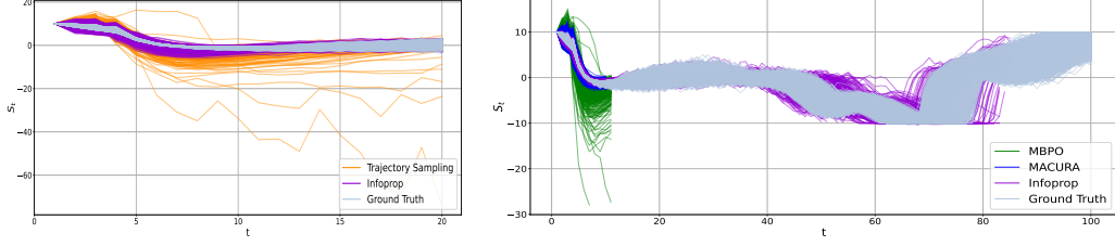
(a) Trajectory Sampling vs. Infoprop (b) MBPO vs. MACURA vs. Infoprop-Dyna Figure 4: Predictive quality of rollouts in the 11 th state dimension of MuJoCo hopper. (a) Rollouts according to Trajectory Sampling (TS) and Infoprop. (b) Rollout schemes of MBPO and MACURA based on TS compared to Infoprop-Dyna.
