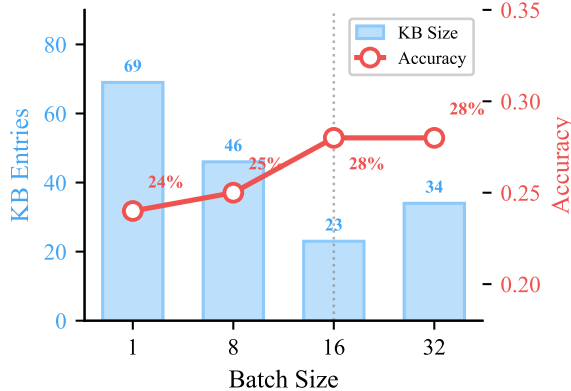
Figure 3: Effect of batch size on KaggleDBQA. Batch size 16 achieves optimal balance: 28% accuracy with only 23 KB entries vs. 24% accuracy with 69 entries at batch size 1.
