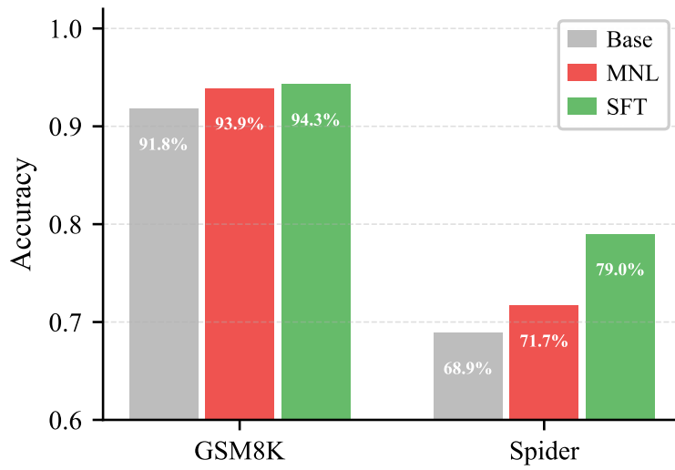
Figure 5: MNL vs. SFT on Qwen3-8B. On GSM8K, MNL (93.9%) nearly matches SFT (94.3%). On Spider, SFT (79.0%) leads, but MNL (71.7%) improves over Vanilla model (68.9%) without parameter updates.
