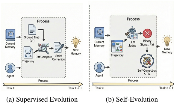
Figure 2: Comparison of the two operating regimes in MNL. (a) Supervised Evolution relies on explicit ground truth ( y^* ) for direct trajectory correction. (b) Self-Evolution leverages a proxy verifier (LLM Judge) to generate binary utility signals, enabling the agent to evolve solely from interaction experience without accessing ground truth labels.
