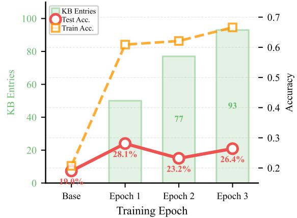
Figure 4: Effect of training epochs on KaggleDBQA. Single-epoch achieves optimal test accuracy (28.1%) with 50 KB entries. Multiple epochs cause cross-epoch overfitting: test accuracy drops to 23.2% at epoch 2 while training accuracy rises to 62.1%, demonstrating the memory overfits to training patterns.
