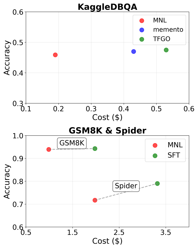
Figure 6: Cost-accuracy trade-off. Top: On KaggleDBQA, MNL achieves 45.9% accuracy at $0.19, while Memento reaches 47.0% accuracy at $0.43 (2.3× cost). Bottom: On GSM8K/Spider, MNL approaches SFT accuracy at 40% lower cost.
