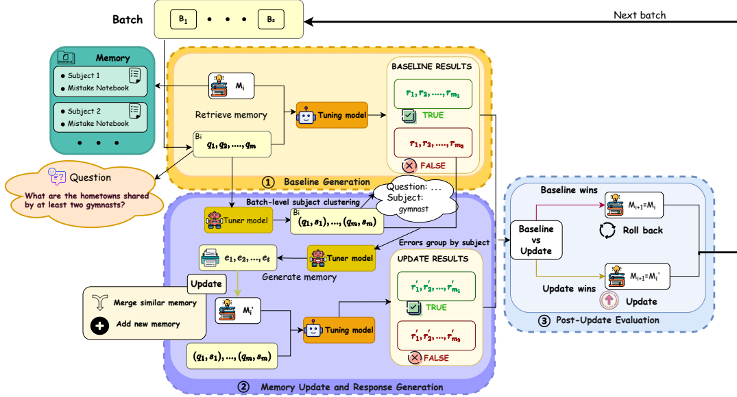
Figure 1: Overview of Mistake Notebook Learning (MNL). By utilizing a Tuning Model (the agent being improved) and a Tuner Model (the supervisor analyzing errors), the whole process consists of three steps: 1) Baseline Generation — The Tuning Model produces initial responses with the current prompt and memory to establish a performance baseline. 2) Memory Update and Response Generation — The Tuner Model performs batch-level subject clustering via prompts, analyzes baseline errors, creates structured guidance items, and selectively updates the memory. The Tuning Model then generates updated responses. 3) Post-Update Evaluation — Compare performance before and after the update to assess the effectiveness of the revised memory and decide whether to accept the update.
