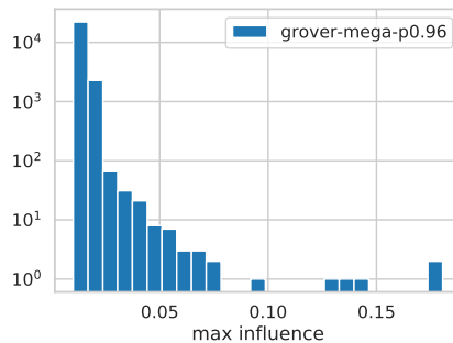
Figure 11: Histogram of max-influence on each generated example by Grover-Mega ( p=0.96 ), from the RealNews training examples.
