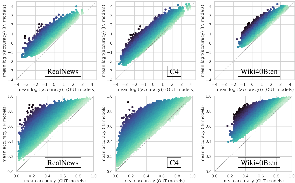
Figure 13: Comparison of directly using the per-token-accuracy vs. taking the logit of the per-token-accuracy. Top row : logit(per-token-accuracy). Bottom row : per-token-accuracy. Figures exactly the same as Figure 7.
