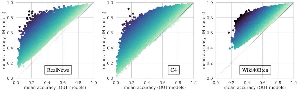
Figure 7: Per-token accuracy of training examples evaluated on IN models vs OUT models.
