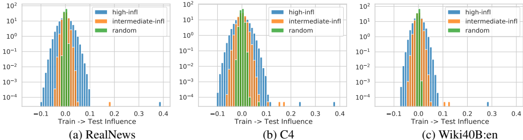
Figure 5: Histogram of the influence of all the training examples on a specific test example for three different test examples. The blue and orange examples have high and intermediate influence from some training examples, as indicated by the outlier values to the right of the each histogram plot. The green (#123456) is a random example, where the influence from all individual training examples are close to zero.
