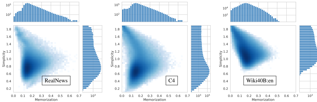
Figure 1: The joint distribution of counterfactual memorization (X axis) and simplicity (Y axis), where simplicity is measured as the overall accuracy for an example across all models. (Histograms are in log-scale).
