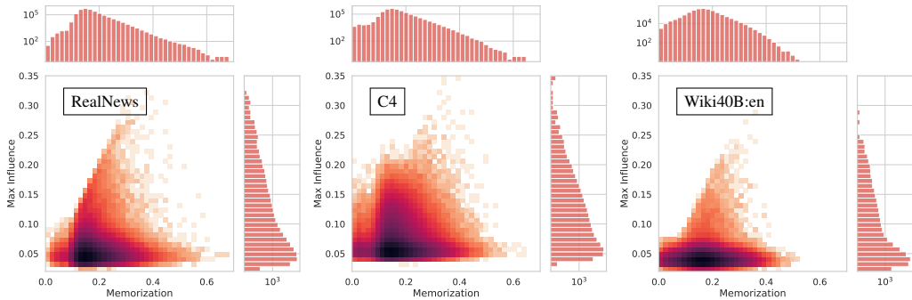
Figure 6: The joint distribution of the memorization score of each training example and its maximum influence on any validation set example. The histograms are in log scale to better visualize the tail of the distributions.
