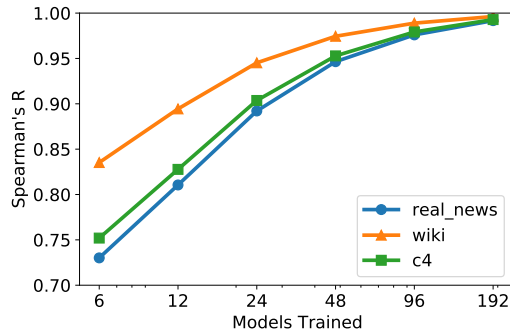
Figure 9: Spearman’s R between memorization rankings from a set of m models and our full set of 400 models. As more models are trained, the ranking changes very little, with the ranking at 192 models having a Spearman’s R of at least 0.992 on all datasets.
