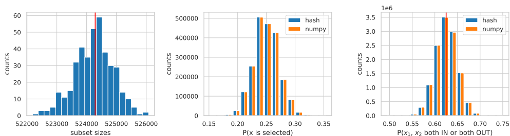
Figure 12: Comparison of hash based subset sampling with numpy.random.choice .
