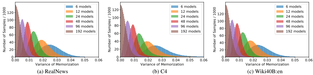
Figure 10: The variance in memorization scores decreases significantly as the number of models increases for all 3 datasets.
