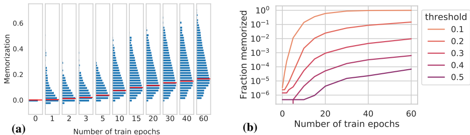
Figure 4: (a) The distribution in memorization of RealNews examples as training progresses. (b) The fraction of RealNews examples with memorization consistently above the specified threshold as training progresses.
