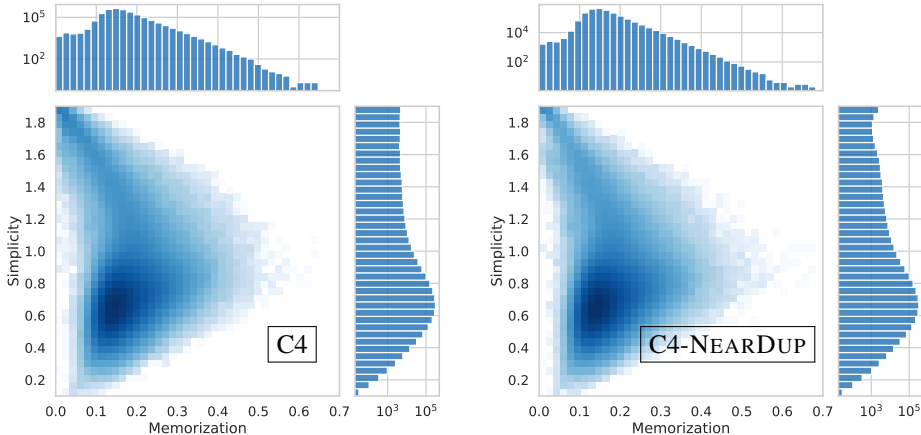
Figure 8: The joint distribution of memorization and simplicity. The histograms are plotted in log scale to better visualize the tail of the distributions.
