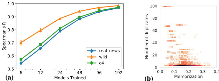
Figure 3: (a) Spearman’s R between memorization rankings from two disjoint sets of m models. The rankings are variable at low numbers of models, but starts to converge at 192 models. All of our other experiments use 400 models. Reported values are averages over up to 10 partitions, with error bars of 10 standard deviations. (b) For RealNews, we plot memorization scores against the number of near-duplicates an example had in the dataset.
