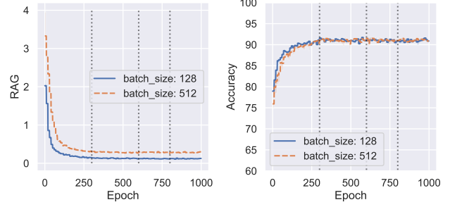
Figure 7. RAG and test accuracy for self-supervised models throughout training, with varying batch size. RAG is computed after every 10 epochs of fine tuning on the classification task. Dashed lines represent learning rate decay by a factor of five
