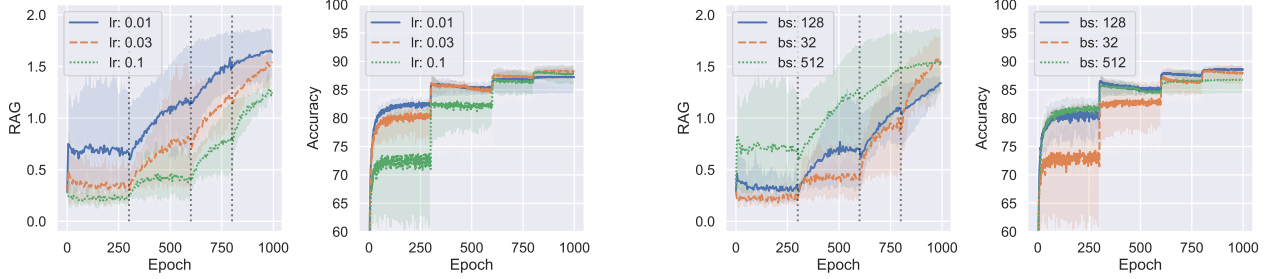
Figure 2. RAG and test accuracy for supervised models throughout training, with varying learning rate (left) and batch size (right). RAG is computed after every 10 epochs of training. Dashed lines represent learning rate decay by a factor of five.
