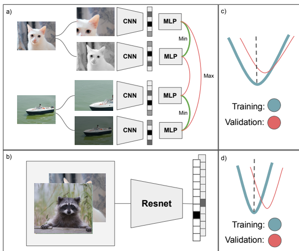
Figure 1. This figure is a visualization of our main hypothesis. Sub-figure (a) represents the workflow for training SimCLR, a SSL approach for learning image representations while (b) is a traditional supervised learning approach. (c) and (d) show hypothetical loss landscapes for SSL and supervised learning respectively. We hypothesize the SSL loss landscape is flatter and less sensitive to shifts in data distribution.
