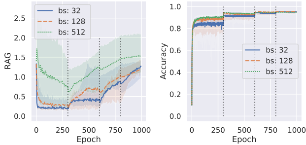
Figure 5. RAG and test accuracy for supervised models throughout training, with varying batch size. Dashed lines represent learning rate decay by a factor of five.
