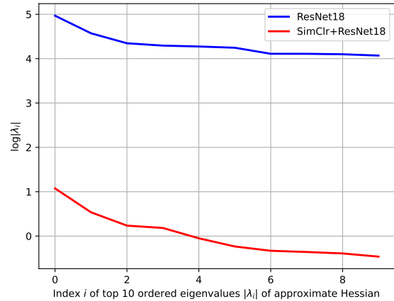
Figure 4. Top 10 log-eigenvalues of approximate Hessian for loss landscape on training data. Supervised model trained using CL representations yields lower magnitudes of eigenvalues, suggesting CL helps models find solutions in lower curvature regions. Magnitude of top eigenvalues for fine-tuned classifier reduce at a quicker rate relative to baseline model.
